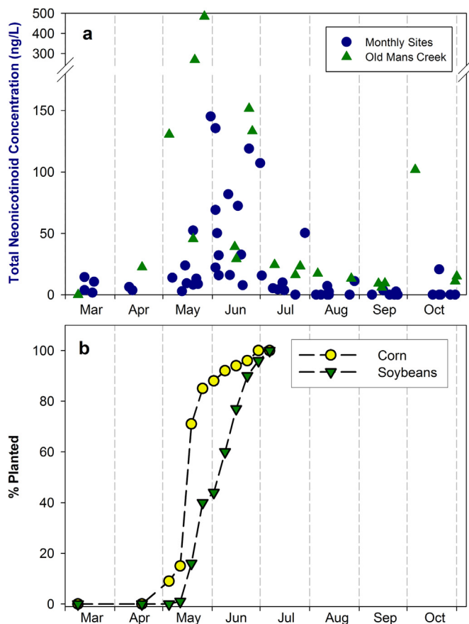
Fig. 6. Comparison of (a) total neonicotinoid concentrations (clothianidin + thiamethoxam + imidacloprid; ng/L) versus date sampled (Old Mans Creek had storm directed sampling so it is separated from the other eight sites that were sampled monthly) and (b) percent of corn and soybeans planted in Iowa (USDA, 2013).
