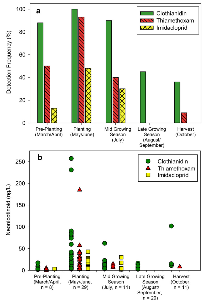
Fig. 5. Summary of (a) detection frequencies and (b) detected concentrations of the three most common neonicotinoids in 79 water samples collected from nine Iowa streams over the 2013 growing season. The number of samples (n) during each time period is listed with the detected concentrations (b).
